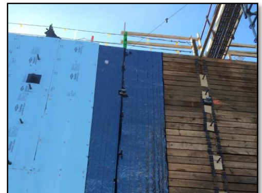
Blindside Membrane Installation
