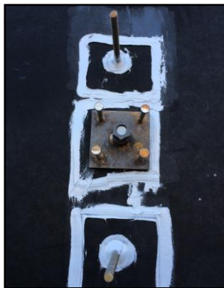
Blindside Membrane detail work
