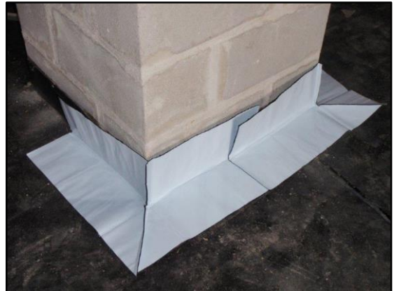
Underslab Membrane Installation with Column Boot
