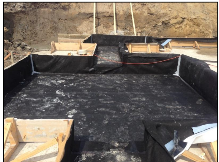
Underseal ® Underslab Membrane installation with Detail Sealant PW ™ detail work at inside corners
